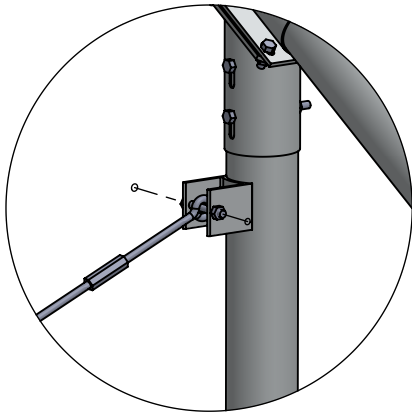
DETAIL BA SCALE 1 : 8
