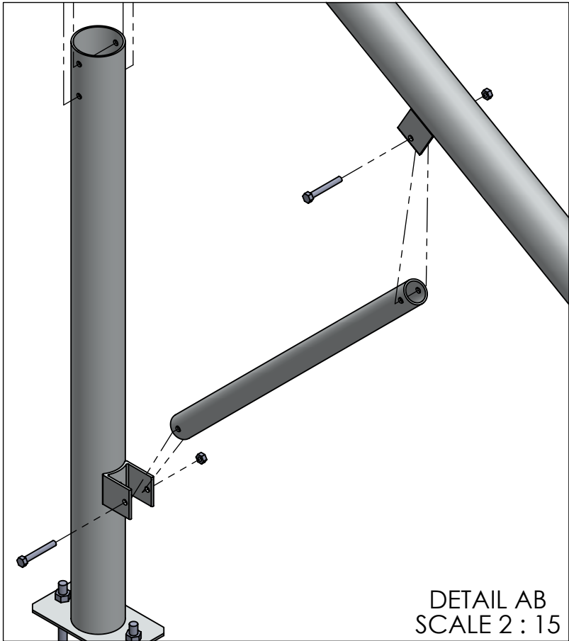
BRACE ASSEMBLY
