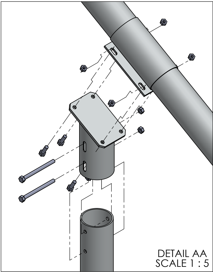
COLUMN TO BEAM ASSEMBLY
